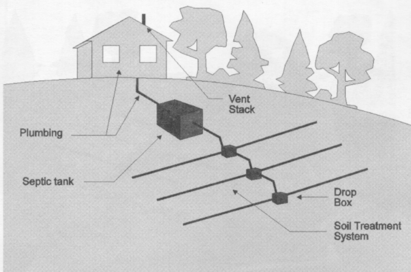
Figure 2. On-site wastewater treatment system components.
