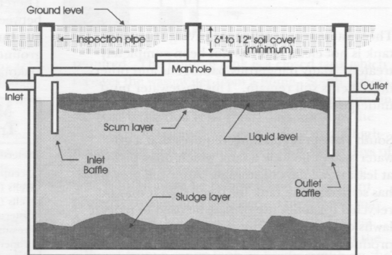
Figure 3. The septic tank.
